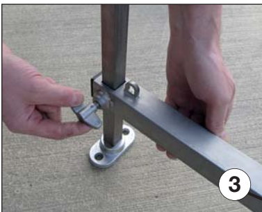
3 Very stable stand with 3 foldable legs. The feet of the legs can be adjusted according to the slope of the site.
